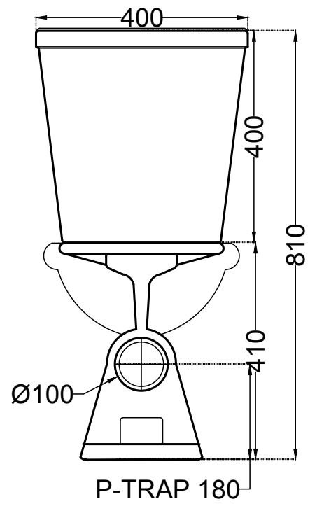
BACK VIEW
