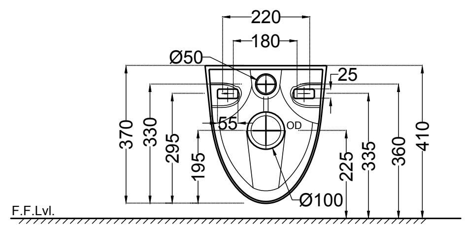
BACK VIEW
