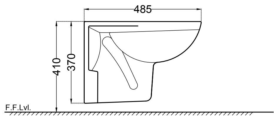
SIDE VIEW
