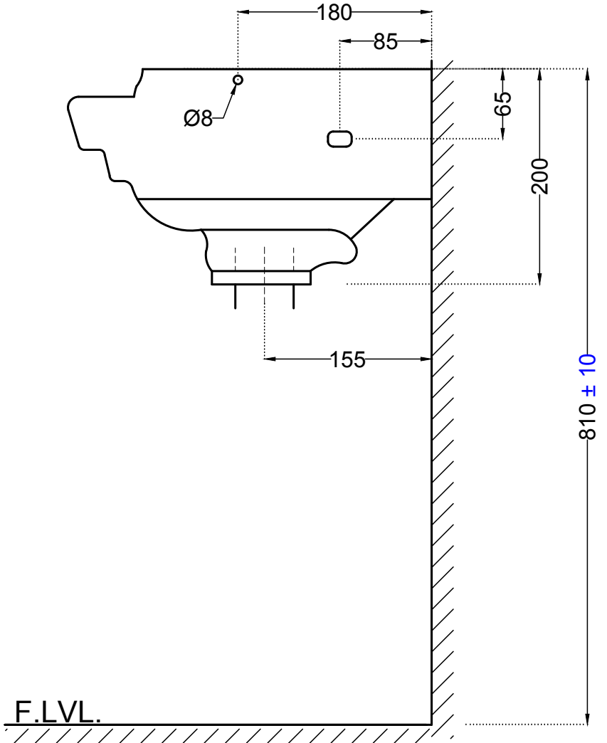
SIDE VIEW
