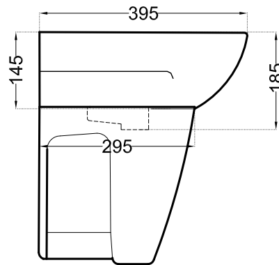
SIDE VIEW WITH PEDESTAL
