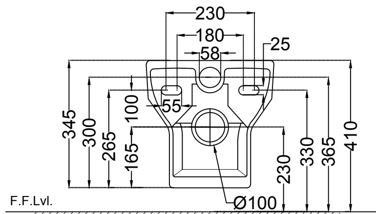
BACK VIEW
