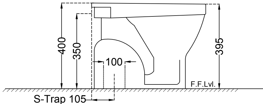
SIDE VIEW
