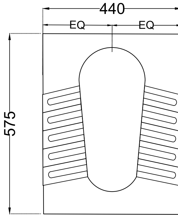
TOP VIEW
