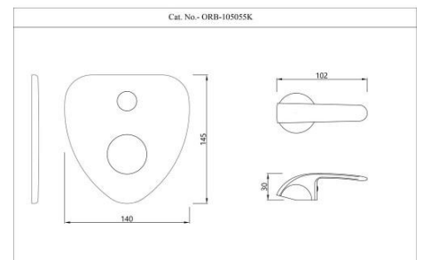
ORB-CHR-105055K Exposed Parts Kit of Single Lever Diverter Price: 650.00 INR
