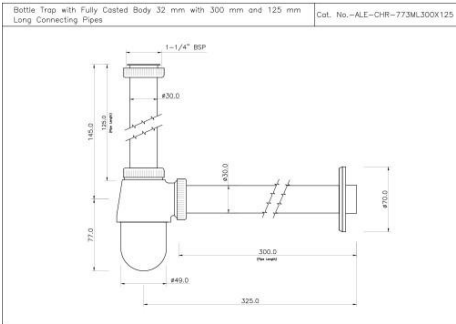
ALE-CHR-773ML300X125 Bottle Trap with Fully Casted Body Price: 1725.00 INR
